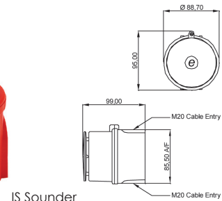
IS Sounder
